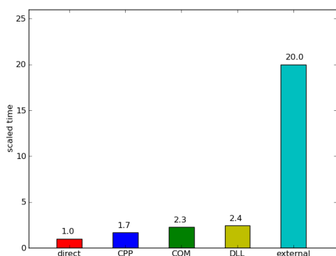
Figure 8. Comparison of scaled run times for the direct solution and the different coupling methods.
