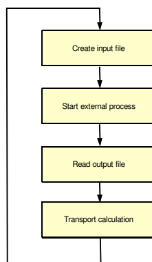
Figure 5. Use of PHREEQC as external process.
