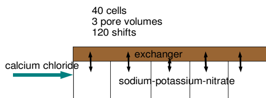
Figure 1. Schematic setup of example problem: The sodium-potassium-nitrate solution is in equilibrium with exchanger and three pore volumes of calcium chloride flush the column.
