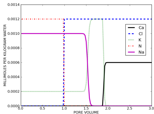
Figure 2. Result of advection modeling with exchange. The concentrations are shown at the outlet of the column.
